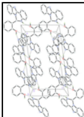
Fig. 3. Part of the crystal structure of the title compound, viewed along the b axis. H atoms not involved in hydrogen bonds (dashed lines) have been omitted for clarity. Only the major disorder component is shown.
