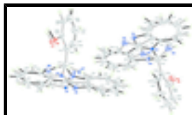
Fig. 1. The molecular structure of the title compound showing 50% probability displacement ellipsoids for non-H atoms. All components are shown.
